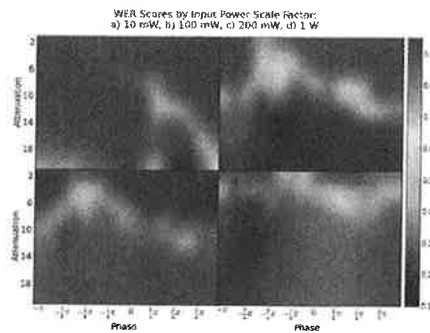
Figure 2: Word error rate for the spoken digit task in the (attenuation, phase) plane for different input peak powers. All the self-loops contain 5 virtual neurons.
