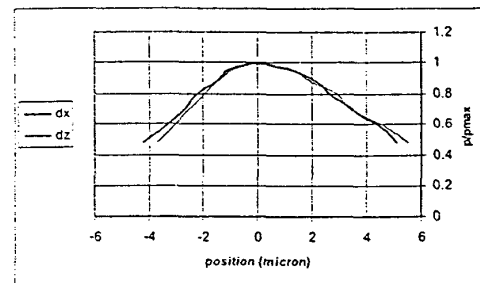
Figure 6 : lateral alignment tolerances
