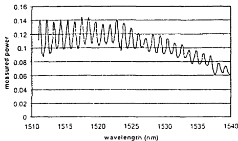
Figure 4: measurement result : P_{out}/P_{in} vs. wavelength
