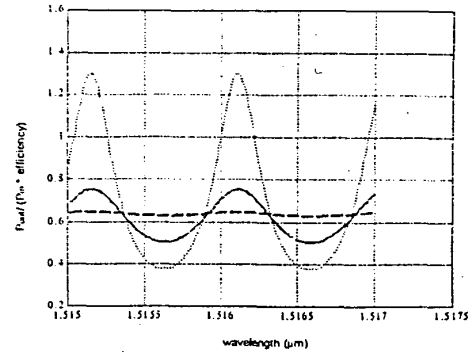
Figure 5: calculation of normalized cavity transmission for different grating reflections
