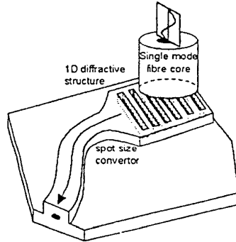
Figure 1: sketch of fibre coupler principle
