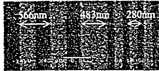
Figure 3: detail of grating (SEM top view)
