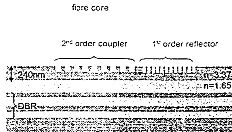
Figure 2: cross section
