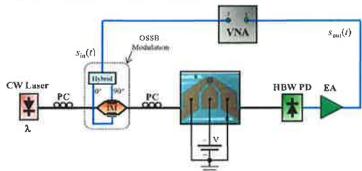
Fig. 1. Sketch showing the experimental setup.
