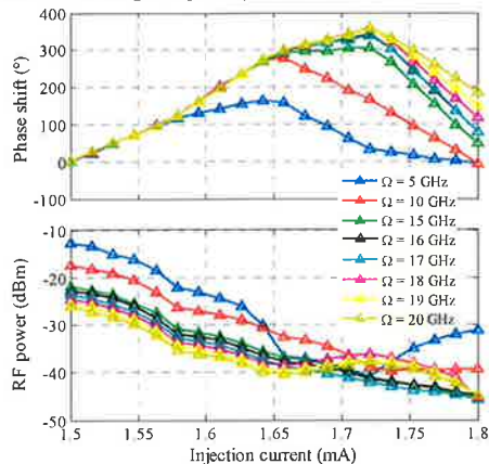
Fig. 3. RF phase shift and power as a function of the injection current for different modulating frequencies.
