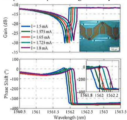
Fig. 2. Gain and phase transfer functions with the injection current.
