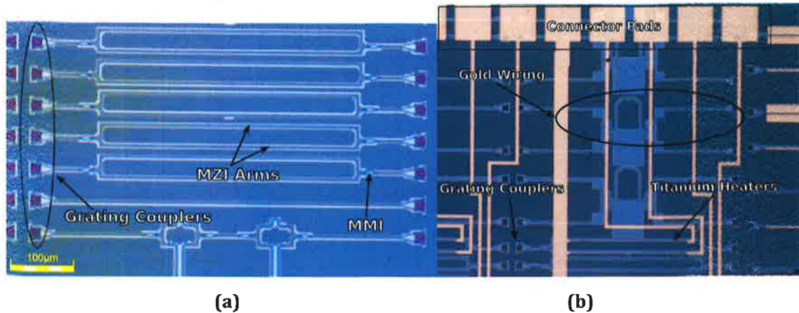
Fig. 25. Microscope image of the integrated MZI (a). Microscope image of the circuit after the processing of the heaters (b).
