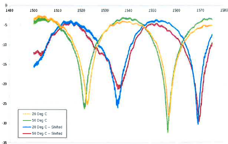
Fig. 2. Spectrum of the transmission of the MZI filter in two different ambient temperatures, 20°C and 50°C, with and without the use of the heaters to shift its operating point.
